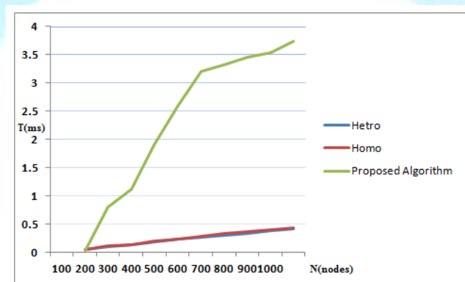
Figure 2. Time T of Homogeneous, Heterogeneous and Proposed algorithm V/S number of nodes.
