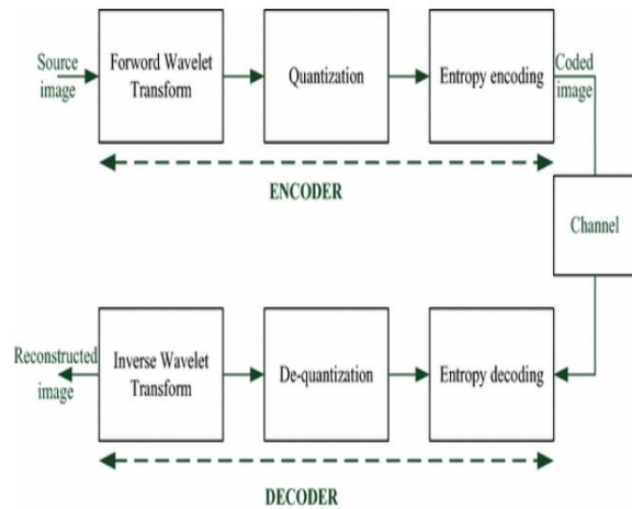
Figure 3: Functional Block Diagram of Jpeg 2000 Encoder
