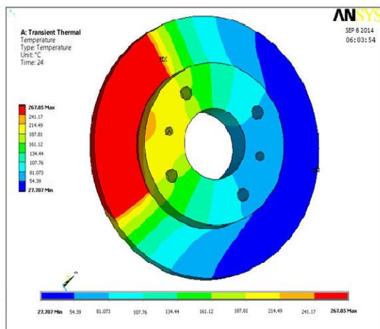
Fig 1.9: Temp.distribution solid stainless steel disc
