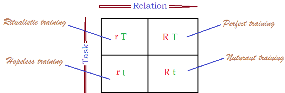
Figure 2: Task-Relation interaction
