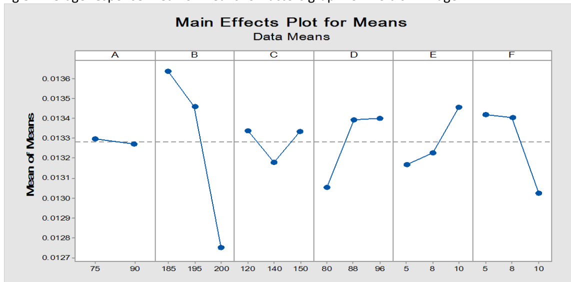
Fig.5. Average response Mean of means for factors graph for mold shrinkage
