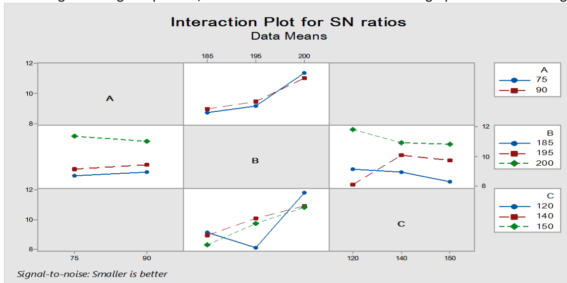
Fig.3. Average response S/N ratio of Interaction of AXB and BXC graph for mold shrinkage
