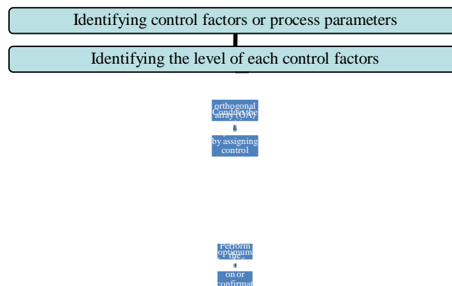
Fig1. Taguchi methodology
